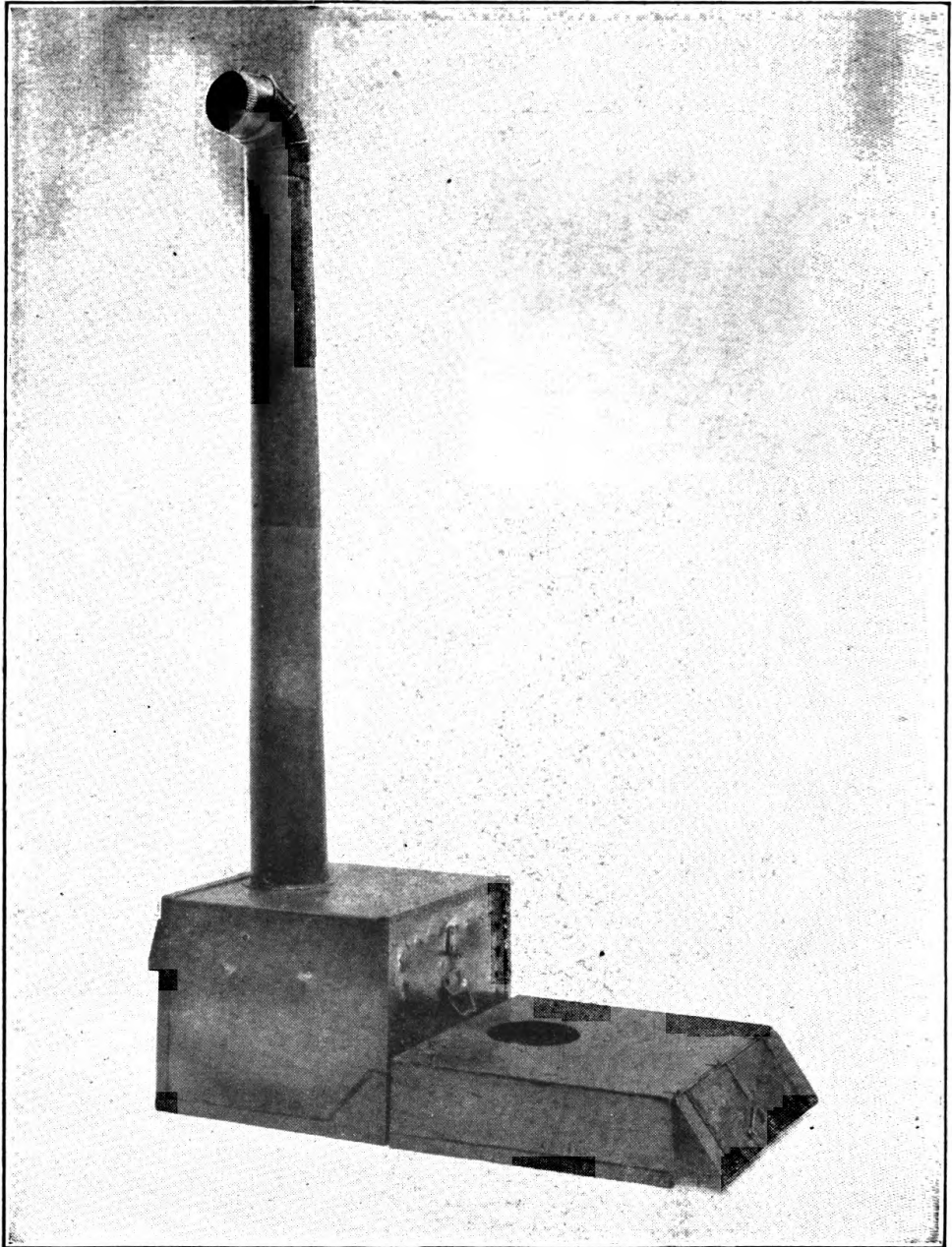
FIGURE 28.—Field range No. 2, set up, rear and right side, with boiling plate.
